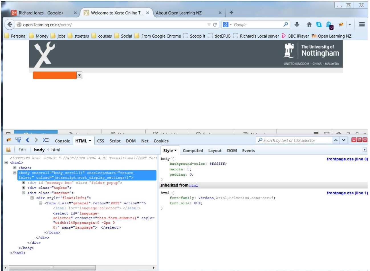
Screenshot 1:
